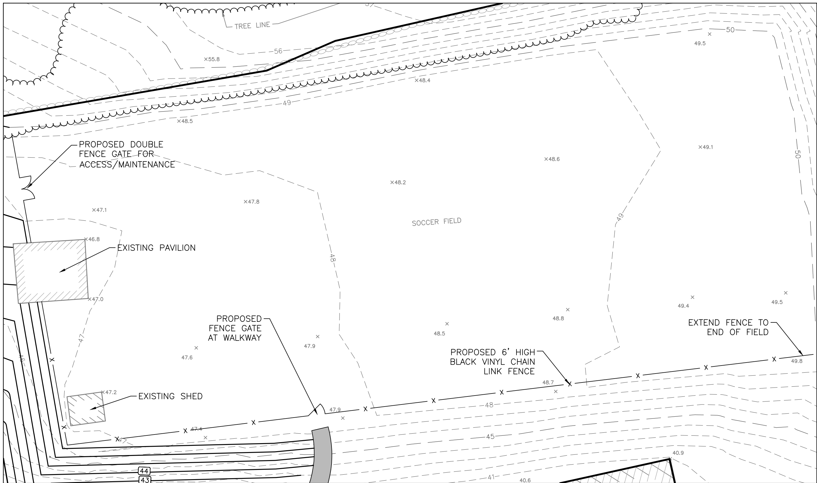
MULTI-PURPOSE FIELD – FENCE PLAN 1" = 20'
